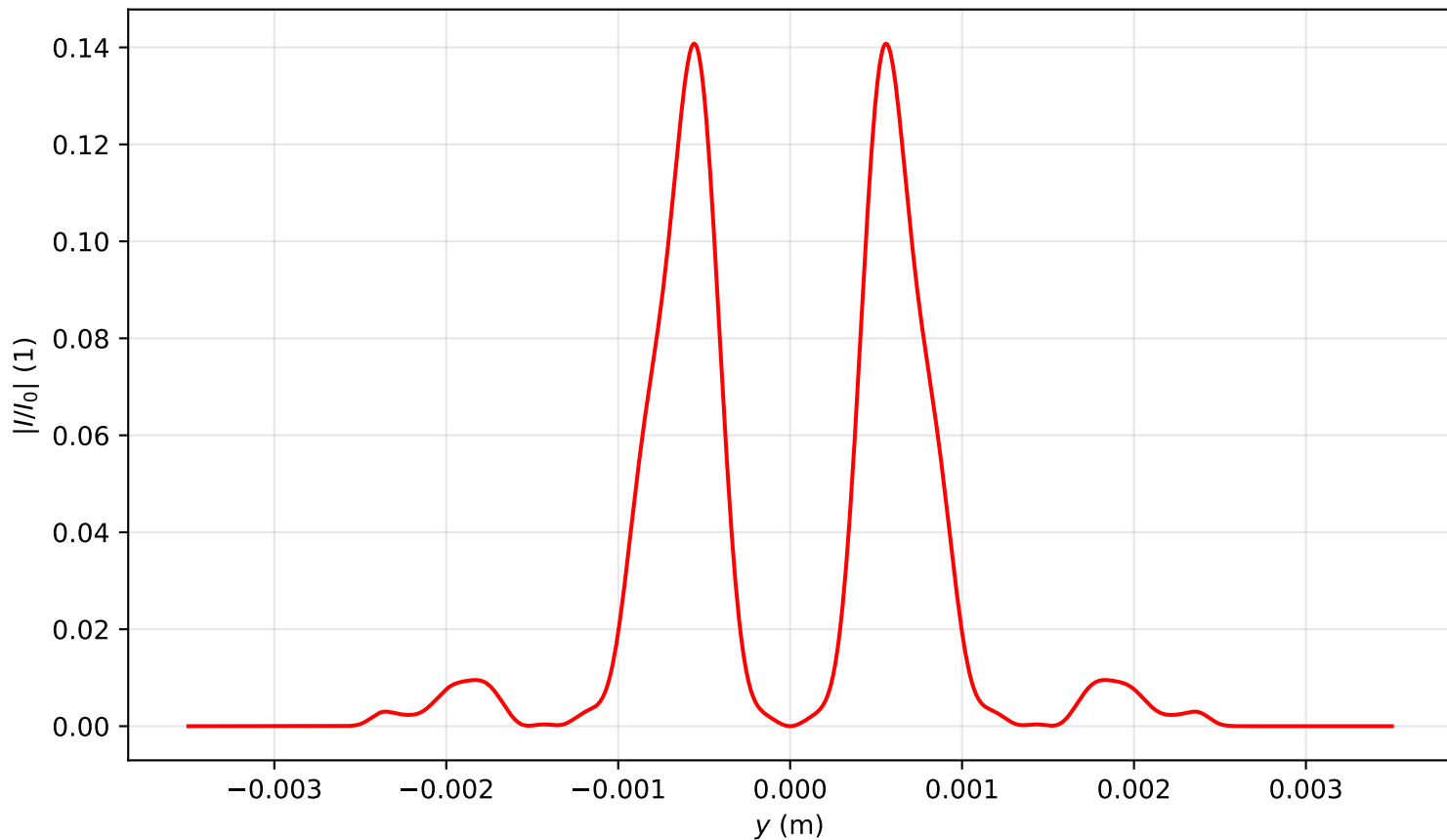
Intensity profile I(x=0, y, z=1.990)/I_0 , P_{in}=5.0P_{cr} , artificial time
